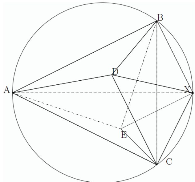
Fig 2: Flat tetrahedron (A,B,C,X) created.
