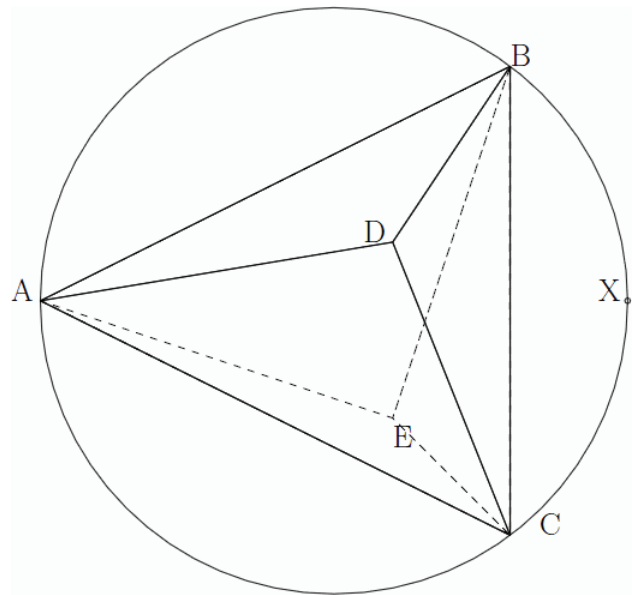
Fig 1: Point X at circumspheres (A,B,C,D) and (E,C,B,A)
